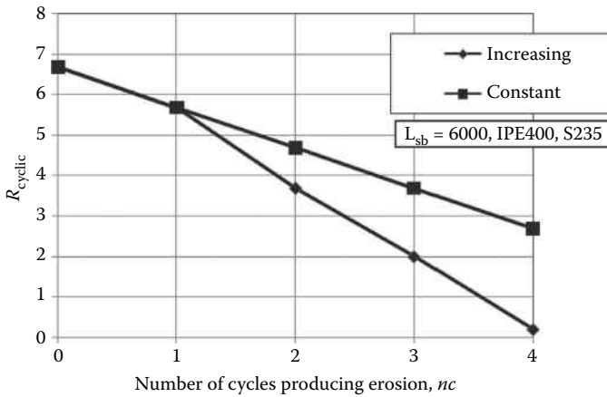
Figure 5.66 Influence of loading type on the available cyclic member ductility.
