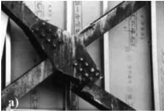
Figure 1.30 Collapse of bolted connections in bracings. (Gioncu, V., Mazzolani, F.M. 2002: Ductility of Seismic Resistant Steel Structures . Spon Press, London; after Fischinger, M. 1997: EASY, Earthquake Engineering Slide Information System. FGG-IKPIP Institute Slovenia.)
