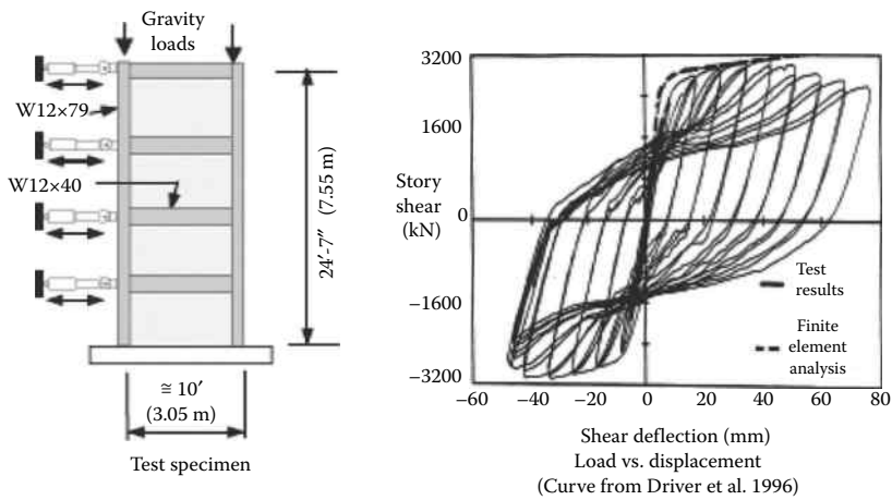
Figure 4.58 The model tested by Driver et al. (1997).
