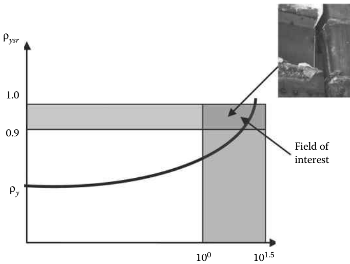
Figure 5.111 Influence of strain rate on yield ratio.
