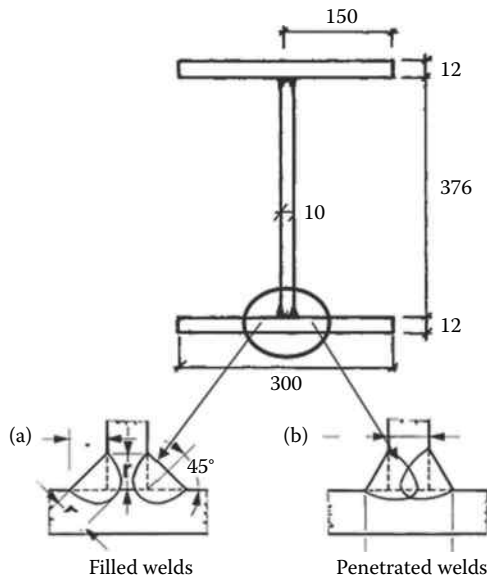
Figure 5.38 Welded profile types: (a) Filled welds; (b) penetrated welds.
