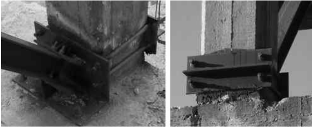
Figure 4.10 Diagonal brace-to-RC end connection. (Della Corte, G., Mazzolani, F.M. 2006: In Proceedings of the 2nd FIB Congress , Naples, Italy, 5–8 June.)
