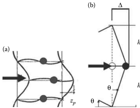
Figure 5.110 Modeling of story drift.
