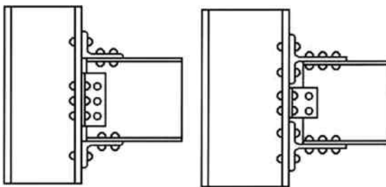
Figure 2.6 Standardized riveted steel frame connection used after 1920. (After Roeder, C.W. 2002: Development of performance-based seismic design criteria for steel moment frames. In 4th National Conference on Steel Structures (eds. D.E. Beskos, D.L. Karakalis, A.N. Kounadis), Patras, 24–25 May, 346–358.)
