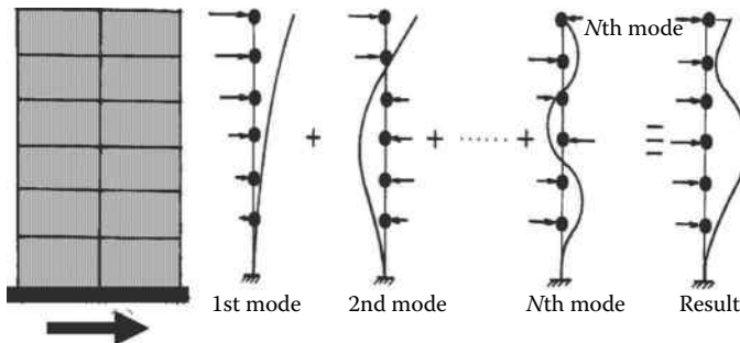
Figure 5.80 Vibration approach.
