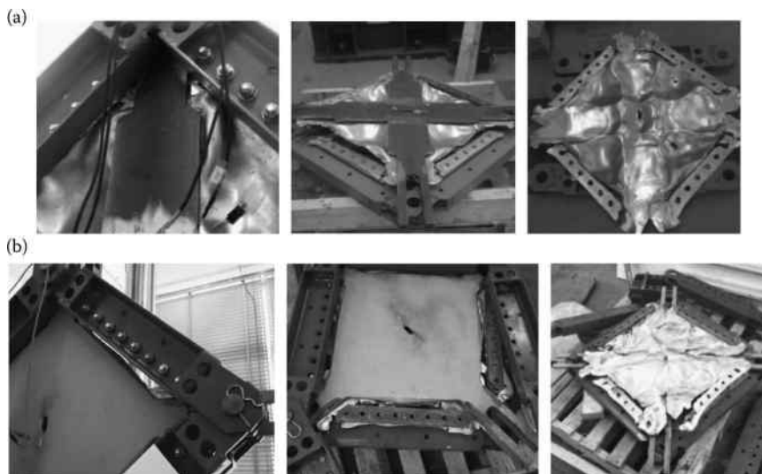
Figure 4.98 Collapse modes of tested specimen: (a) p-BIP and (b) t-BIP.
