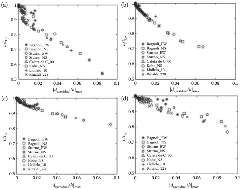
Figure 6.21 Normalized fire resistance rating versus maximum value of the residual interstory drift angle: (a) P-ULS; (b) P-SLS; (c) S-ULS; (d) S-SLS.
