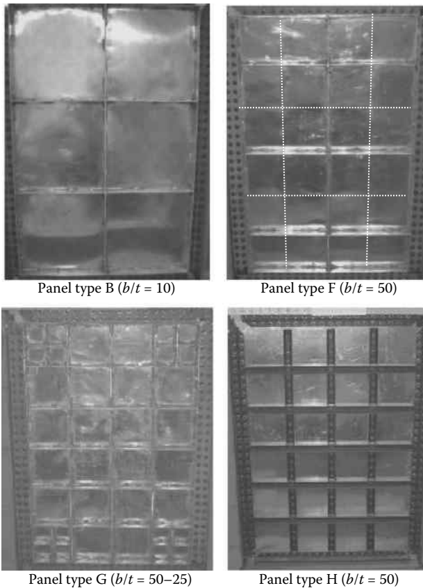
Figure 4.80 Geometrical configuration of tested full bay shear panels.
