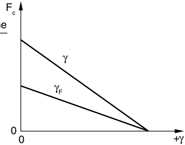
Figure 2.12 Negative chamfer angle means less increase in force than with a negative rake angle without chamfer
