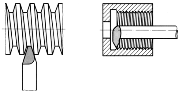
Figure 7.13 Workpiece, on which the turning tool is allocated for thread turning a external thread, b internal thread
