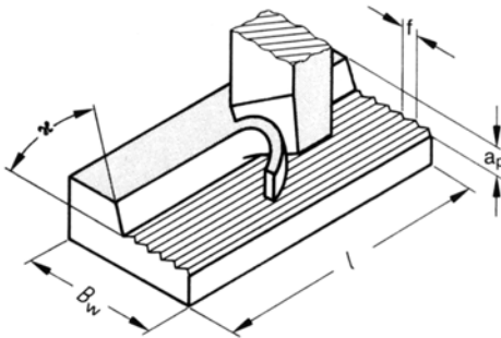
Figure 8.3 Cutting parameters for planing l workpiece length, B_w workpiece width, f feed, a_p depth of cut, i tool cutting-edge angle
