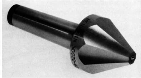
Figure 7.23 Lathe carrier (rotating gripper) to carry pipes (photo by Neidlein, Stuttgart)
