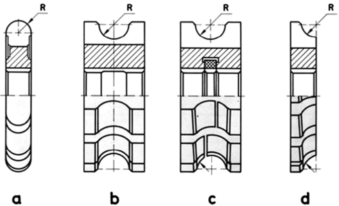
Figure 11.37 Circular milling cutter of the former type
