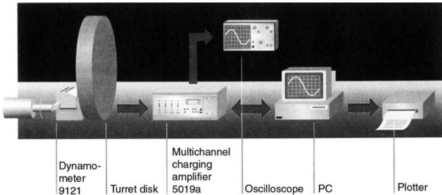
Figure 22.2 Force measurement chain during turning (Courtesy of Kistler AG, Winterthur/Switzerland)
