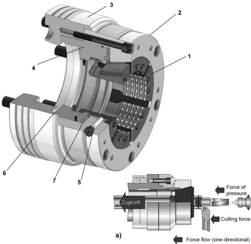
Figure 7.24 SPANNTOP nova chuck 1 clamping chuck, 2 chuck body 3 spindle flange, 4 pulling mechanism, 5 radial fixing, 6 clamping reserve with stroke limit, 7 opening path with stroke limit, a) chuck mounted in and fixed at the main flange (photo by Hainbuch GmbH, Erdmannhäuser Str. 57, 71672 Marbach)
