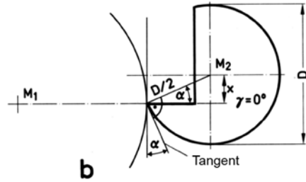
Figure 7.38b Formation of the tool orthogonal clearance for the wheel turning tool. M_1 workpiece centre, M_2 tool centre, D \varnothing of the formed wheel, x offset in height, \alpha tool orthogonal clearance
