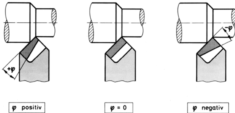
Figure 7.42 Halved cone angle of the chip breakers
