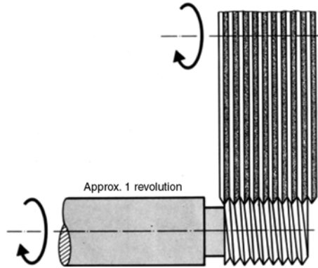
Figure 13.9 Plunge-thread grinding with multi-edged wheel
