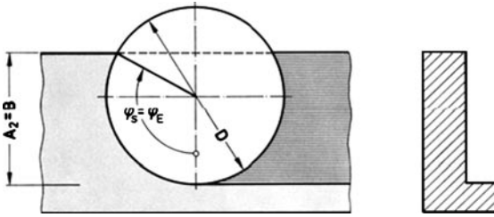
Figure 11.18b Principle of face milling
