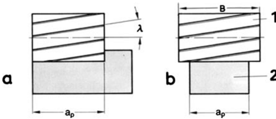
Figure 11.16 Width of cut a_p during peripheral milling, 1 milling cutter, 2 workpiece Figure a: a_p defined by milling cutter width, Figure b: a_p given by workpiece width
