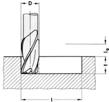
Figure 11.23 Paths during groove milling
