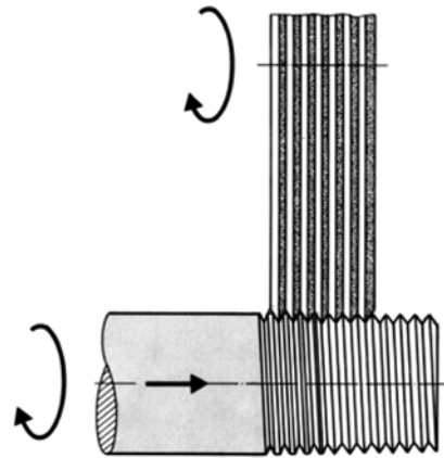
Figure 13.8 Longitudinal grinding of a thread with multi-edged wheel
