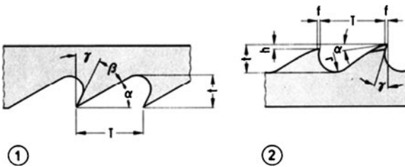
Figure 10.10 Angles and pitch for saw tooth; 1 band saw blade; 2 circular saw blade; clearance angle; wedge angle; rake angle; T pitch; t tooth depth ( t = 0,4 T )
