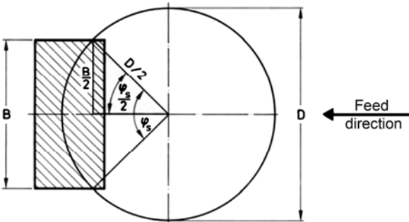
Figure 10.6 Length of cut at circular saw blade, l = \text{arc length to } \varphi_s
