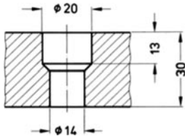
Figure 9.48 Plate with stepped hole
