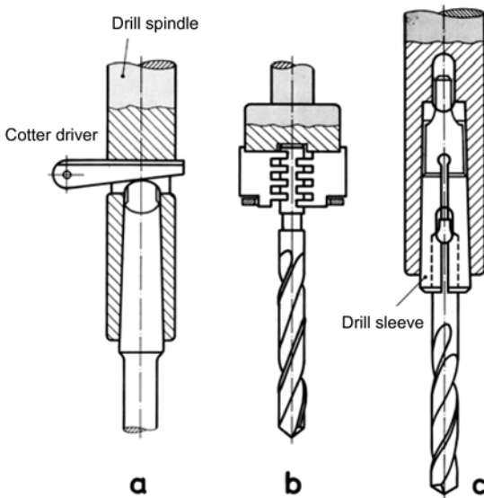
Figure 9.16 Variants of clamp twist drills a) drill with Morse taper in drill spindle, b) drill with parallel shank in the chuck, c) drill with parallel shank and tang in drill sleeve
