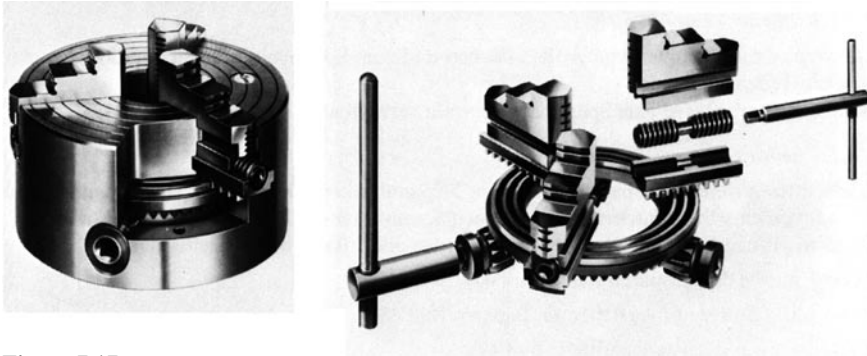
Figure 7.17 Spiral ring chuck with adjustable jaws (photo by Röhm, Sontheim)
