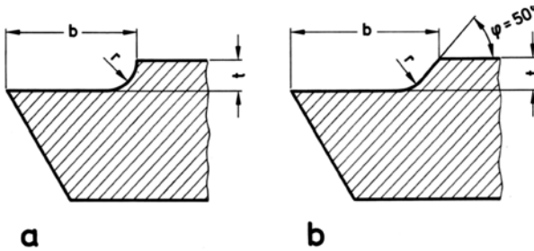
Figure 7.44 Dimensions of chip breaker b in mm width, t in mm depth, r in mm radius, \varphi in ^\circ angle of lapping
