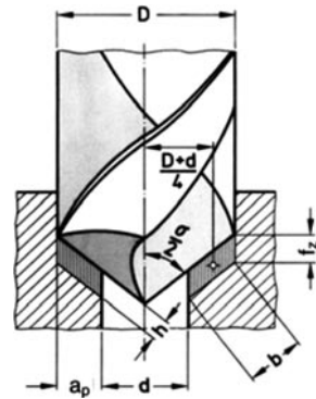
Figure 9.11 Cutting parameters for drilling out
