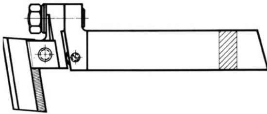
Figure 7.37 Turning tool holder with inserted formed blade a) side view of the holder with blade, b) formed blade for metric threads (photo by Komet Stahlhalter und Werkzeugfabrik, 74351 Besigheim)
