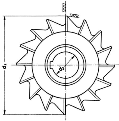
Figure 11.35 Single-angle cutter
