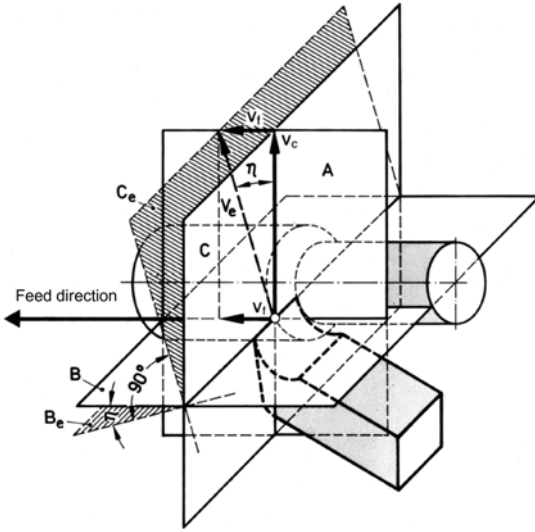
Figure 2.15 Reference planes for the turning tool: A working plane, B tool reference plane, B c working reference plane, C tool cutting edge plane, C c cutting plane, v c cutting speed in primary motion direction, v e cutting speed in working plane, \eta effective cutting speed angle, v r feed rate in the direction of feed motion
