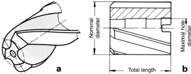
Figure 9.27 Helical counterbore geometries, a) 3-edged helical counterbore, b) 4-edged arbour-type counterbore
