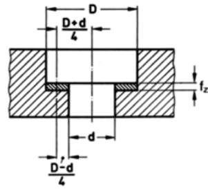
Figure 9.12 Cutting parameters and distances for spot facing
