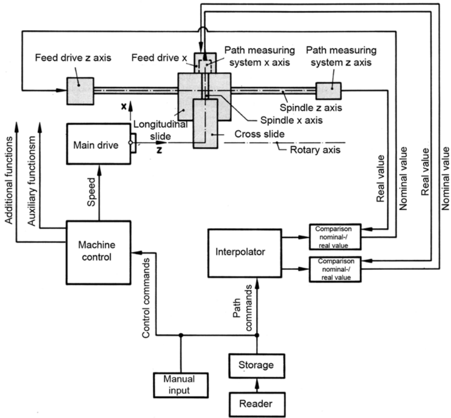
Figure 7.12 Structure of a numerical control for 2- axis turning [according to Dräger]
