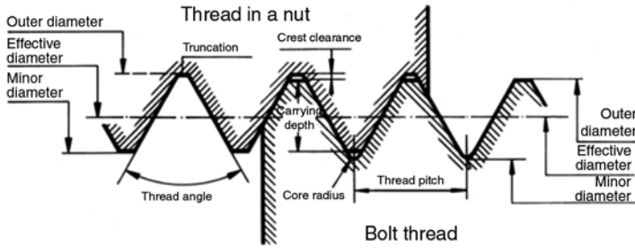
Figure 9.44 Thread profiles for bolts and nuts
