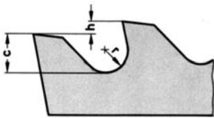
Figure 12.11 Tooth offset
