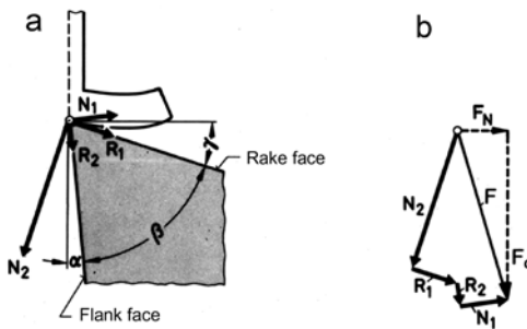
Figure 2.17a + b Effective forces on the wedge. N_1 normal force on the rake face; N_2 normal force on the flank face; R_1 frictional force on the rake face; R_2 frictional force on the flank face; F resultant cutting force
