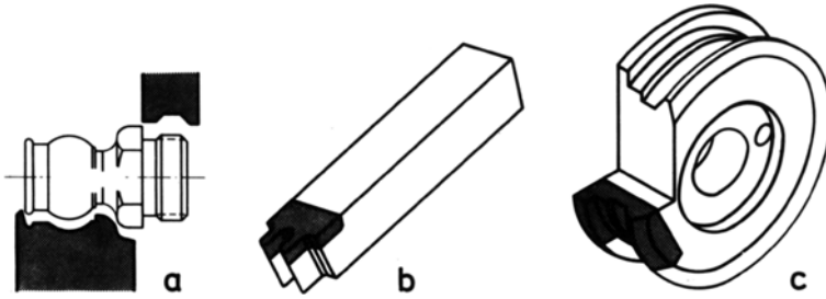
Figure 7.40 a workpiece generated with profile turning tool, b profile turning tool with cemented carbide tip, c profile turning wheel (photo by Hufnagel, Nürnberg)
