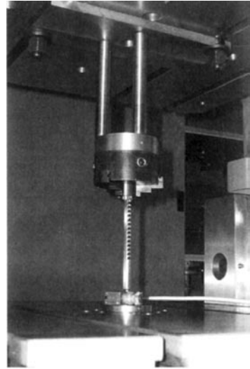
Figure 22.10 Force measurement during broaching (test) (photo by HTW Dresden, practical cutting course)
