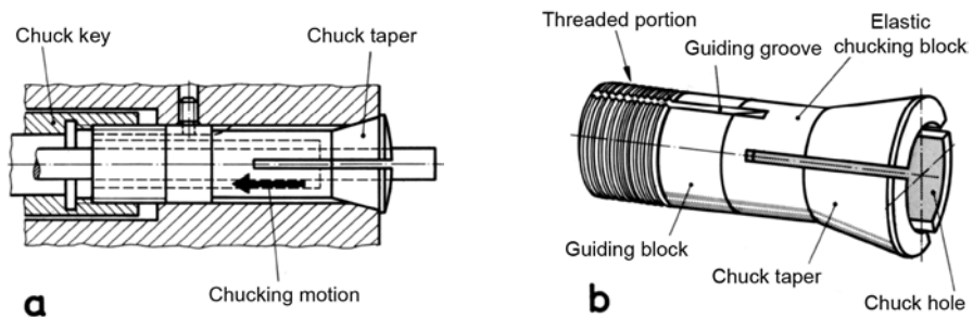
Figure 7.20 a + b a force-locked collet, b exchangeable collet
