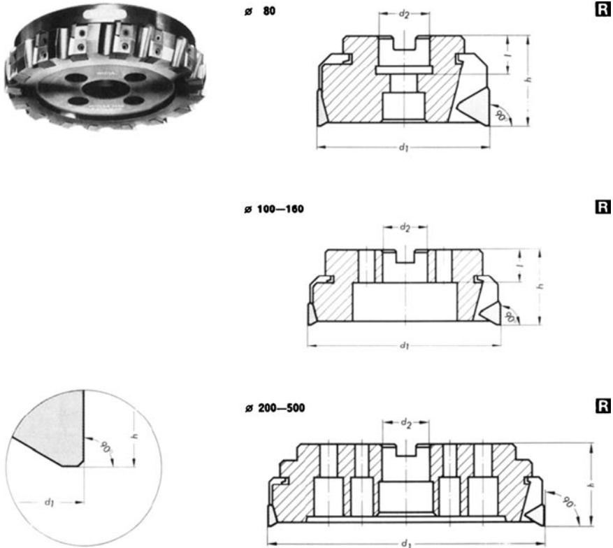
Figure 11.42 Cutter head, designed as corner milling cutter (photo by Krupp Widia-Fabrik, Essen)
