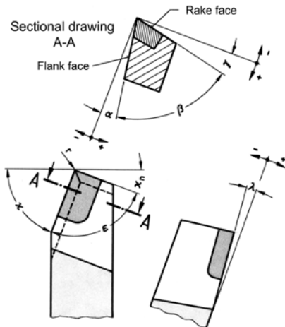
Figure 2.5a Overview showing the most significant angles on the wedge
