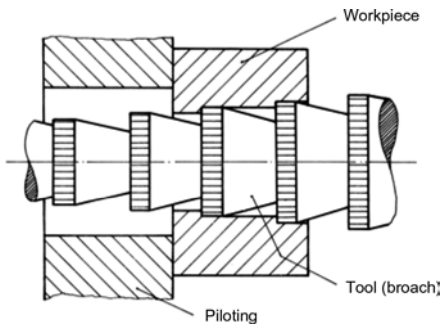
Figure 12.1 Broaching principle
