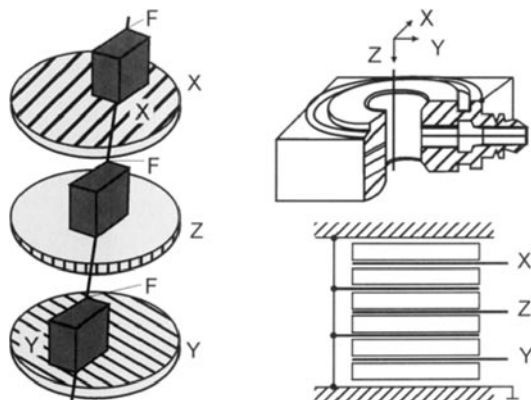
Figure 22.1 View of the principle of a 3-component-dynamometer for cutting force determination (Courtesy of Kistler AG, Winterthur/Switzerland)
