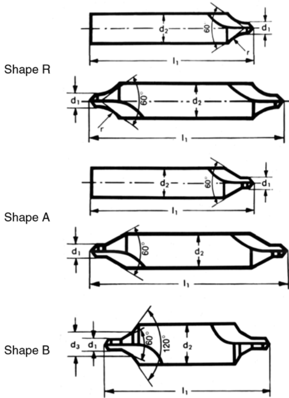
Figure 9.34 Centre drill according to DIN 333 shapes A, B and R (Photo by Günther & Co, Frankfurt)
