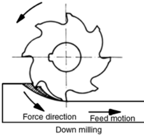
Figure 11.3 Down milling principle, marked force direction is related to the workpiece
