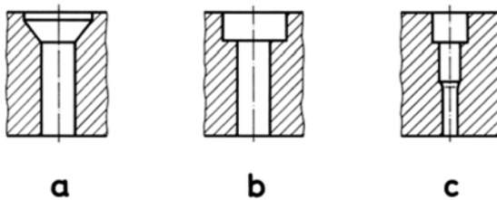
Figure 9.23a – c Counterbores/ countersink generated with multi-cut drills a) for countersunk head screw, b) for fillister head cap screw, c) countersink stepped twice.
