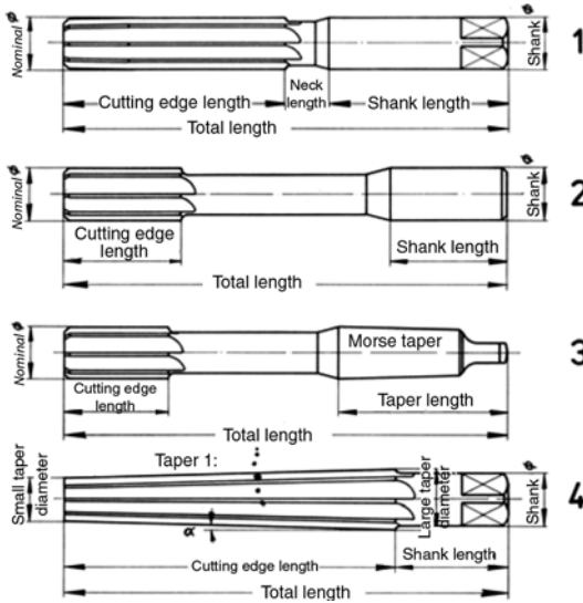
Figure 9.37 Elements of a reamer (body - shank) 1 hand reamer, 2 machine reamer with parallel shank, 3 machine reamer with Morse taper, 4 taper reamer (photo by Boeklenberg Söhne, Wuppertal)
