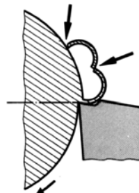
Figure 7.43 Chip flowing against the workpiece surface with negative halved cone angle
