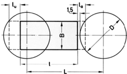
Figure 11.21 Total path L during central face milling
