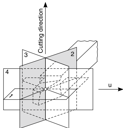
Figure 2.2 Reference system to define the angles for the wedge
