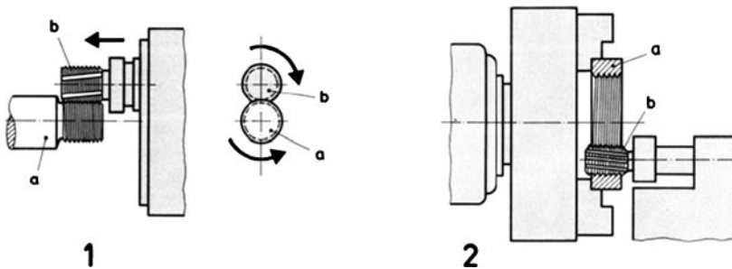
Figure 11.10 1 workpiece and tool configuration during short-thread milling of external threads 2 workpiece- and tool configuration during short-thread milling of internal threads. a workpiece, b mill
