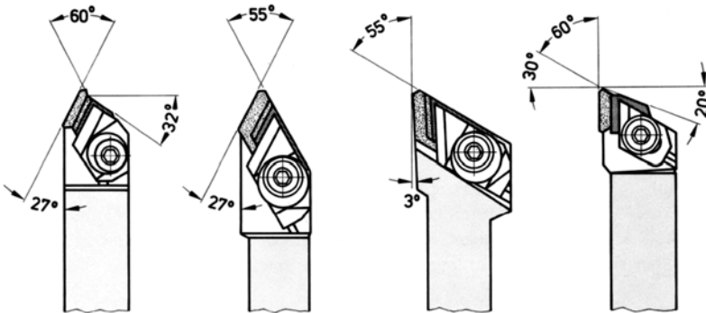
Figure 7.41 Clamp-type tool holders for form turning, for shapes with positive rake angle (photo by Widia-Fabrik, Essen)
