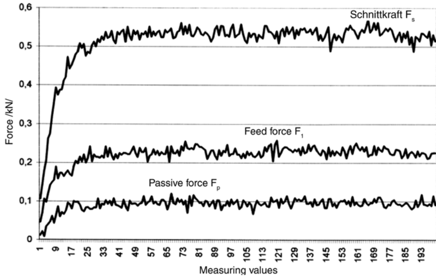
Figure 22.4 Test results for turning k = 70^\circ ; a_p = 2,5 \text{ mm} ; f = 0,112 \text{ mm/rev}
