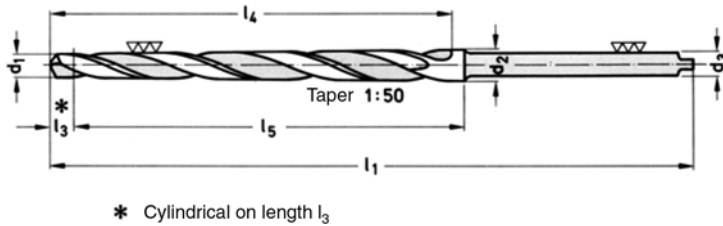
Figure 9.25 Taper pin hole drill (taper 1 : 50)
