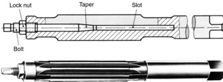
Figure 9.42 Adjustable reamer, adjustable by means of an expansion arbour
