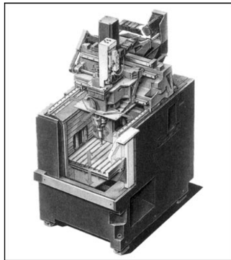
Figure 20.6 Machine bed made as mineral casting (photo byHermle AG, Gosheim)
