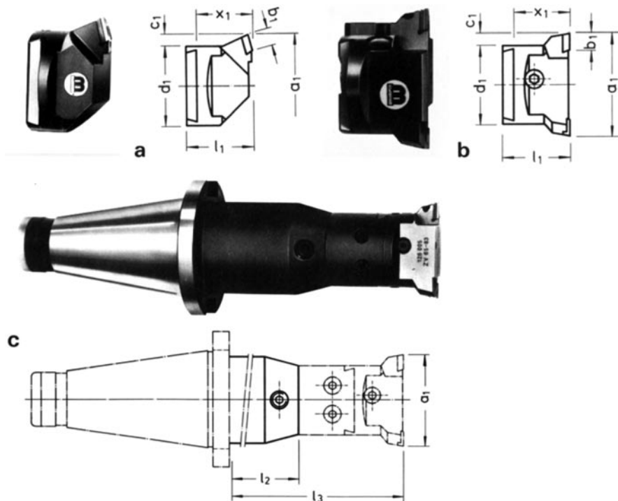
Figure 9.35 Tool heads, a) with one cutting edge, b) with two cutting edges (Photo by Wohlhaupter, Frickenhausen)
