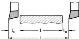
Figure 8.4 Length L in planing
