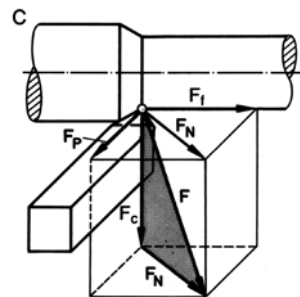
Figure 2.17c Decomposition of the resultant cutting force F in major cutting force F_c and minor force F_N and decomposing the minor force F_N into feed force F_f and passive force F_p
