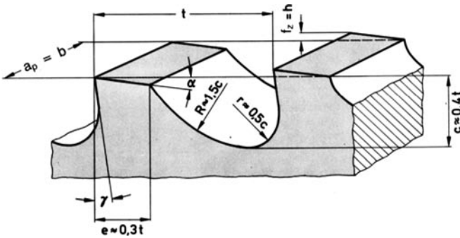
Figure 12.5 Cutting variables during broaching t pitch, e tooth back thickness, c tooth space depth, r rake face radius, f_z stepping of the cutting edges (feed per cutting edge), a_p broach width
