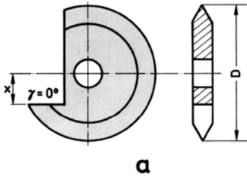
Figure 7.38a Wheel turning tool
