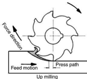
Figure 11.1 Up milling principle, inserted force direction relates to the workpiece
