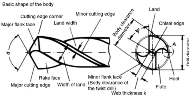
Figure 9.17 Twist drill body, \sigma = point angle, \psi = chisel edge angle
