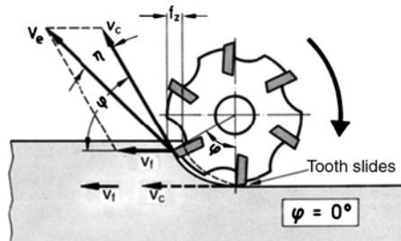
Figure 11.2 Feed motion angle \varphi during peripheral milling in the up milling mode ( \varphi < 90^\circ ), illustrated velocities relate to the tool, v_e effective cutting speed (photo by Sitzmann and Heinlein)
