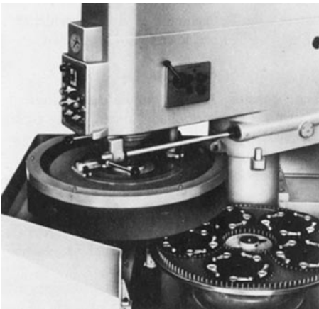
Figure 18.2 Hydraulic two plate-lapping- and precision grinding machine, type ZL 800 H, with planetary driving attachment (photo by Hahn & Kolb, Stuttgart)
