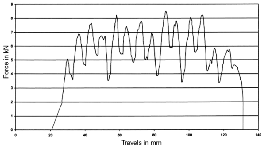
Figure 22.11 Test results gained for broaching (Broach made of high-speed steel; for a groove width 5 mm; length l = 170 mm; internal sleeve diameter d = 16 mm; tooth number z = 16 ; broaching depth = 1,4 mm)
