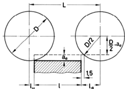
Figure 11.20 Total path L during peripheral milling
