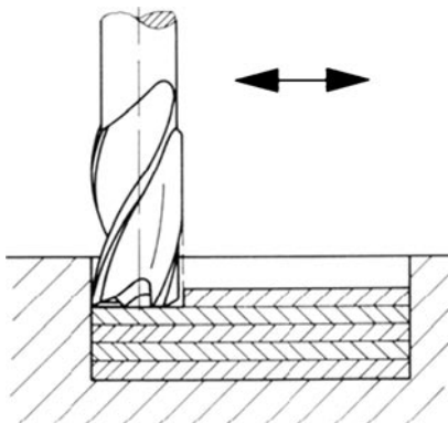
Figure 11.12 Principle of line milling to generate grooves
