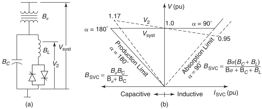
Figure 3.22 An FC-TCR with a step-down transformer and its V-I characteristics.
