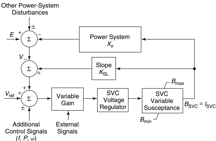
Figure 5.21 The SVC voltage controller with variable gain ( V \approx V_{rated} ).
