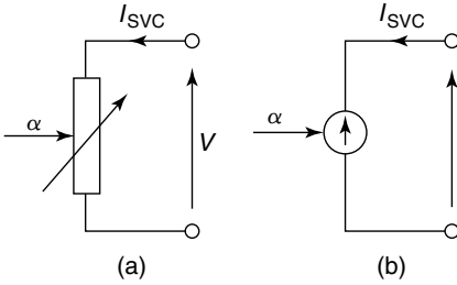
Figure 4.29 Basic static var generator models for small- and large-disturbance studies: (a) the susceptance model and (b) the current-source model.
