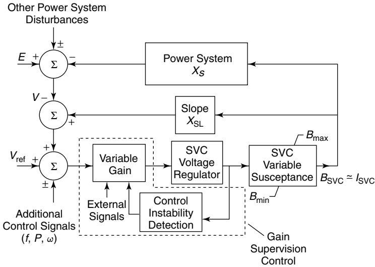
Figure 5.24 The connection of gain-supervisor control to the SVC voltage-control system ( V \approx V_{rated} ).
