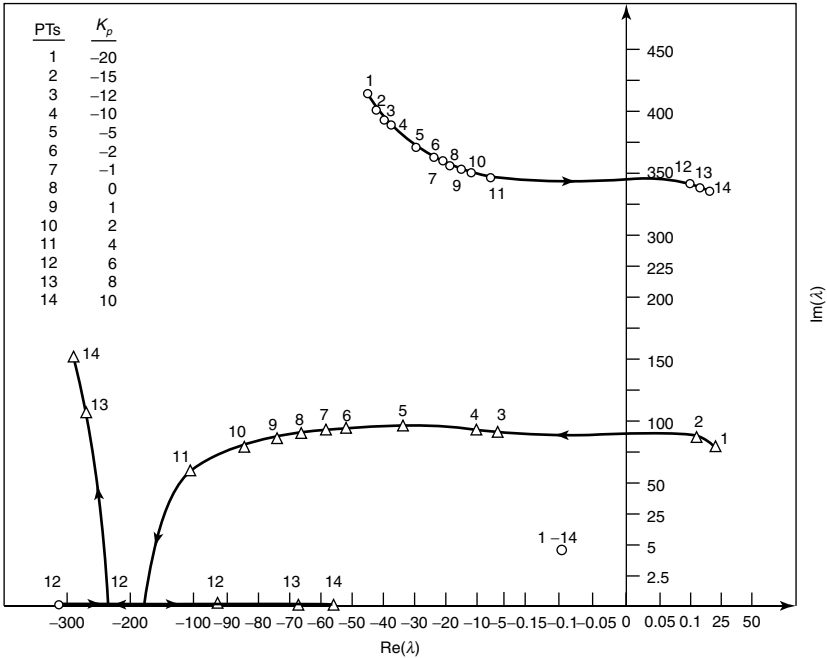
Figure A.3 (a) The root loci of a detailed model with varying K_I ( K_P = 0 ) and (b) the root loci of a detailed model with varying K_P ( K_I = 1200 ).
