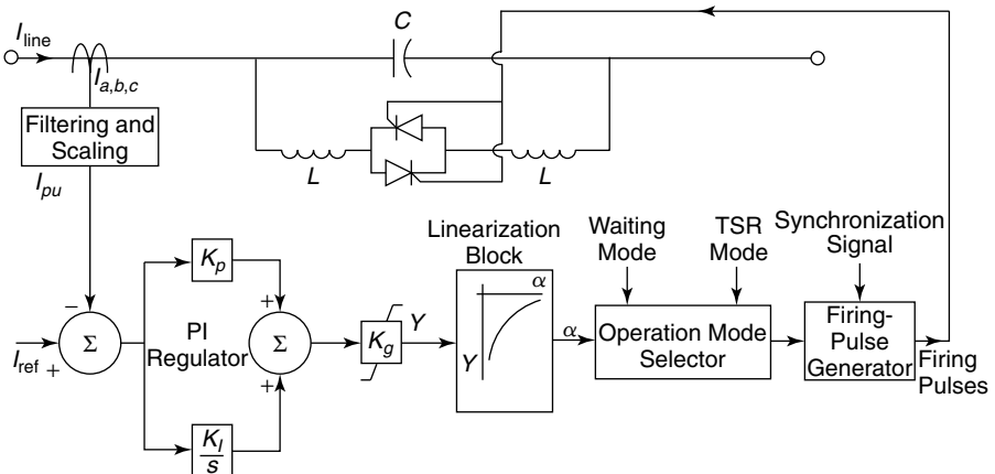
Figure 8.2 A TCSC constant-current (CC) controller model.
