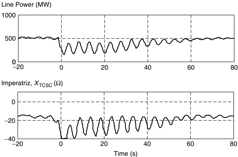
Figure 8.36 Tripping of 300-MW generator in Tucuruí, with the lead-lag POD in Imperatriz and the Serra da Mesa disabled.
