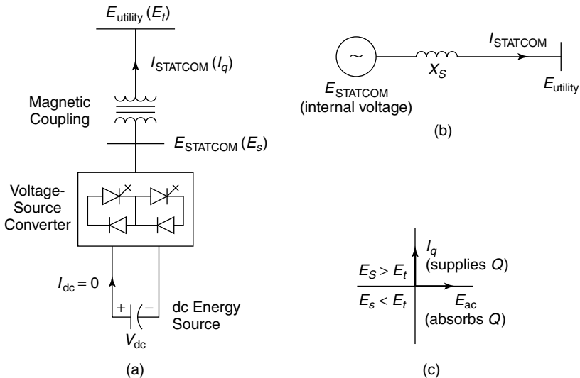
Figure 10.1 The STATCOM principle diagram: (a) a power circuit; (b) an equivalent circuit; and (c) a power exchange.
