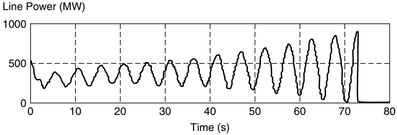
Figure 8.35 Tripping of 300-MW generator in Tucuruí, with the lead-lag and phasor PODs both disabled.
