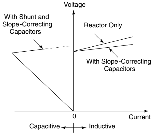
Figure 3.5 The operating characteristics of an SR compensator.
