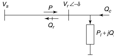
Figure 2.5 The reactive-power balance at the receiving end.
