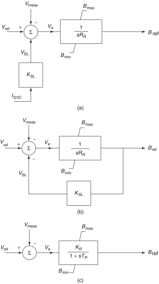
Figure 4.15 Alternative implementations of current droop (slope) in the voltage regulator: (a) an integrator with current-droop feedback; (b) an integrator with susceptance-droop feedback; and (c) a gain–time constant.
