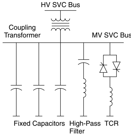
Figure 3.20 An FC–TCR SVC.
