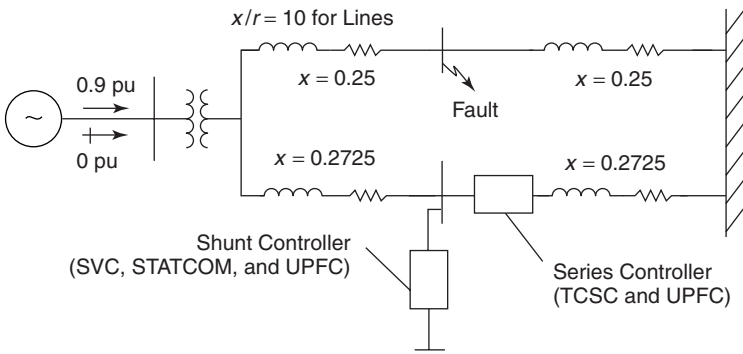
Figure 10.31 A study system for transient-stability evaluation.
