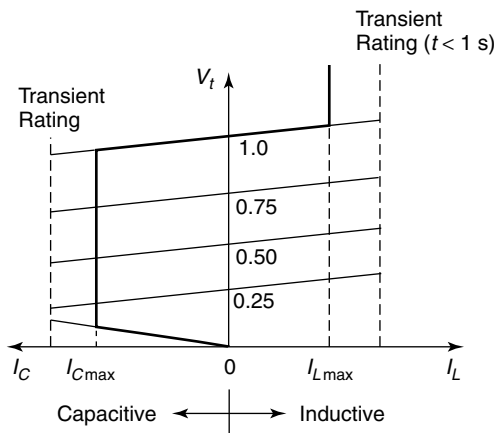
Figure 10.2 The V-I characteristic of the STATCOM.
