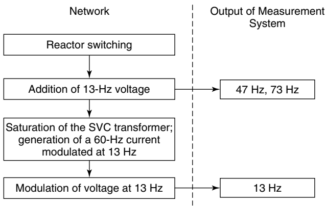
Figure 5.47 Explanation of the addition/modulation phenomenon.
