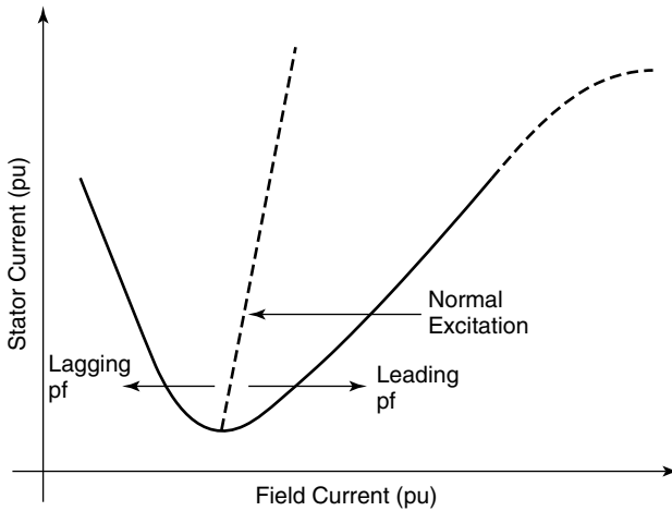
Figure 3.1 The relation between stator current and field current in the synchronous condenser.
