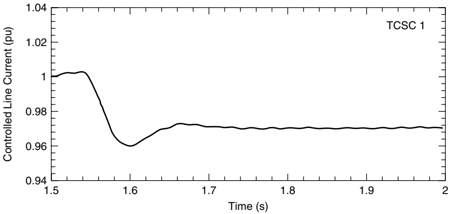
Figure 9.33 An independently optimized TCSC controller.
