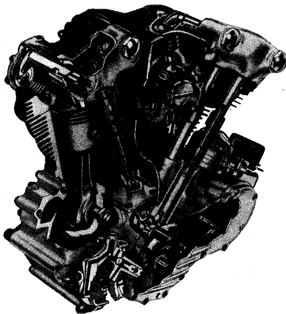
Figure 1-13 Harley-Davidson two-cylinder, air-cooled, overhead valve "Knucklehead" motorcycle engine first introduced in 1936. The 45° V engine had displacement of 60 cubic inches with 3.3125 inch bore and 3.500 inch stroke. Operating on a four-stroke cycle with a compression ratio of 7:1 the engine was rated at 40 bhp at 4800 RPM. Ignition was by Harley-Davidson generator-battery system. Photograph courtesy of the Harley-Davidson Juneau Avenue Archives. All rights reserved. Copyright Harley-Davidson.
