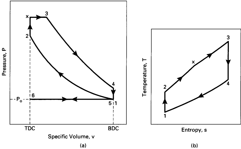
Figure 3-10 Air-standard Dual cycle, 6-1-2-x-3-4-5-6, which approximates the four-stroke cycle of a modern CI engine on (a) pressure-specific volume coordinates, and (b) temperature-entropy coordinates.
