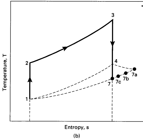
Figure 3-6 Air-standard Otto cycle for engine at WOT, showing process 4-7 experienced by exhaust during blowdown.
