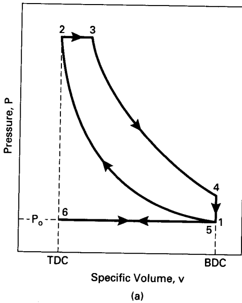
Figure 3-8 Air-standard diesel cycle, 6-1-2-3-4-5-6, which approximates the four-stroke cycle of an early CI engine on (a) pressure-specific volume coordinates, and (b) temperature-entropy coordinates.
