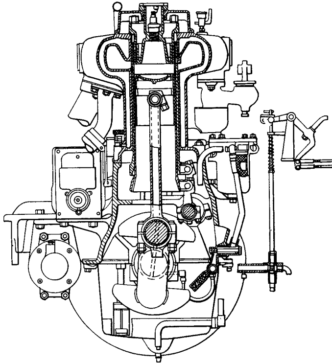
PRINCIPAL PLANTURE OF THE KNIGHT ENGINE
