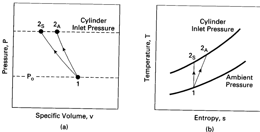
Figure 5-7 Ideal flow process ( 1-2_s ) and actual flow process ( 1-2_A ) through a supercharger or a turbocharger compressor in (a) pressure–volume coordinates, and (b) temperature–entropy coordinates.
